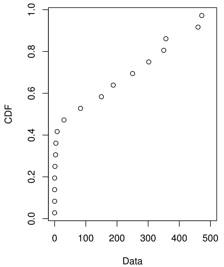
Cumulative distribution
