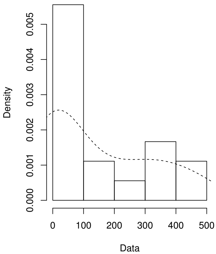
Empirical density
