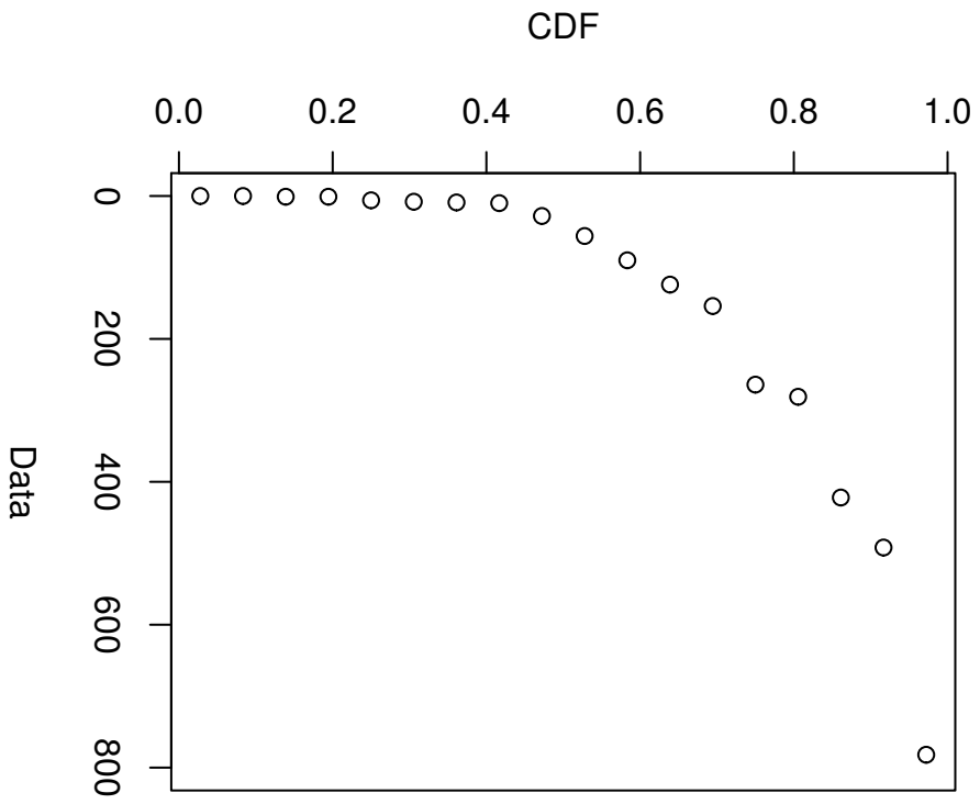
Cumulative distribution
