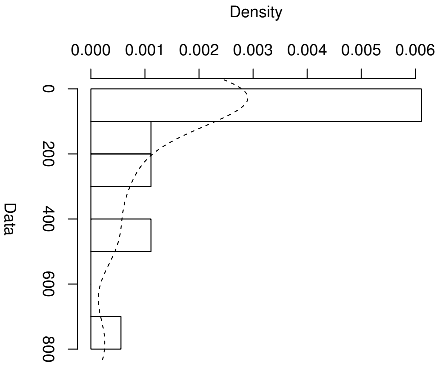
Empirical density
