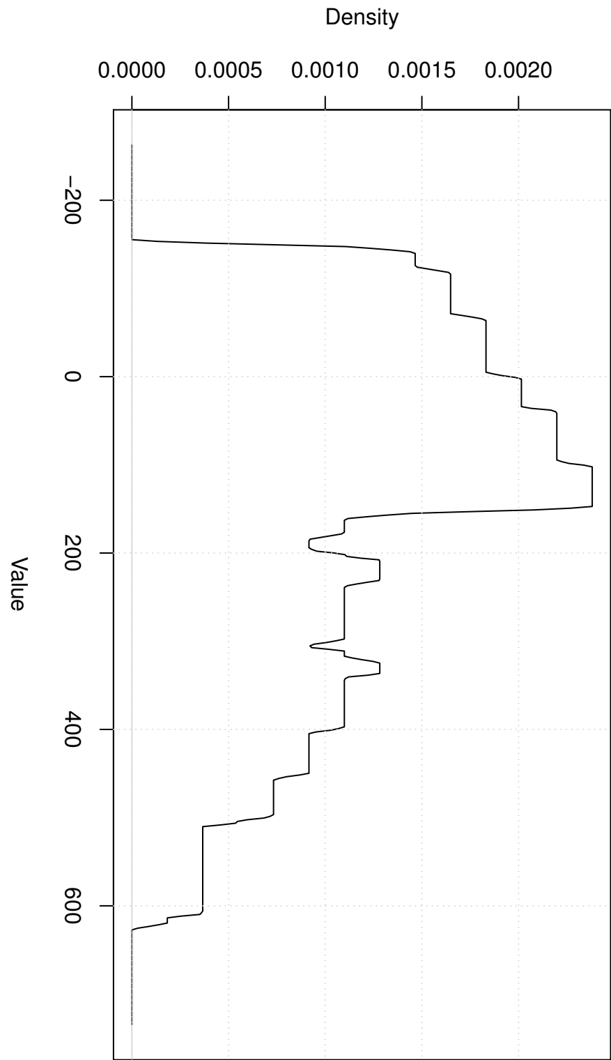
Rectangular Kernel
