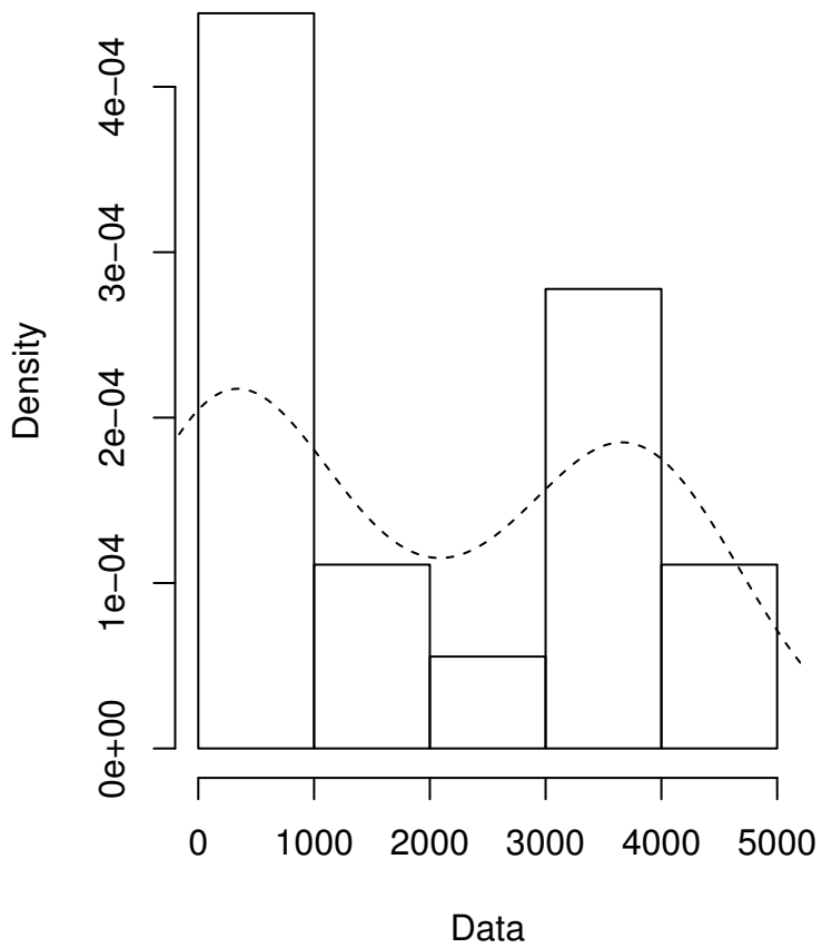
Empirical density
