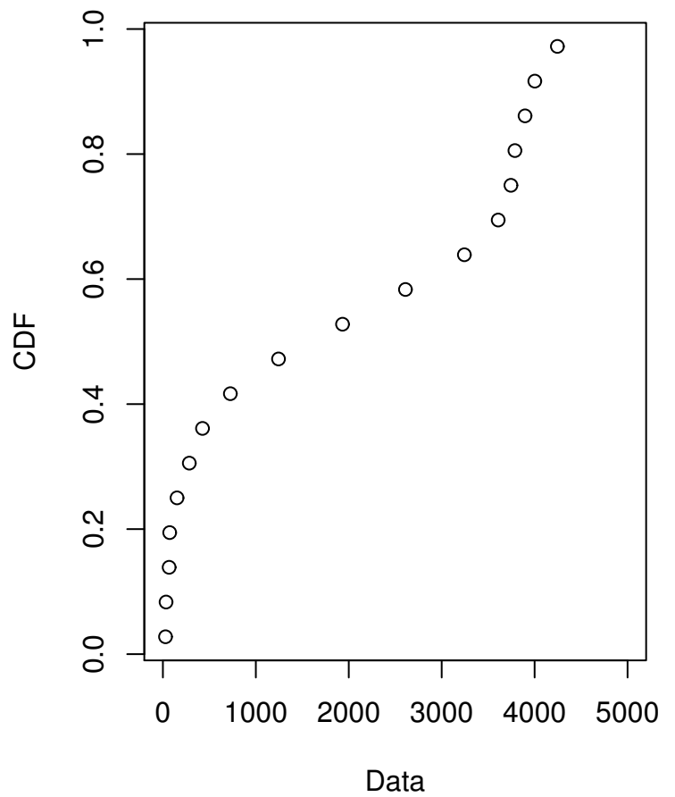
Cumulative distribution
