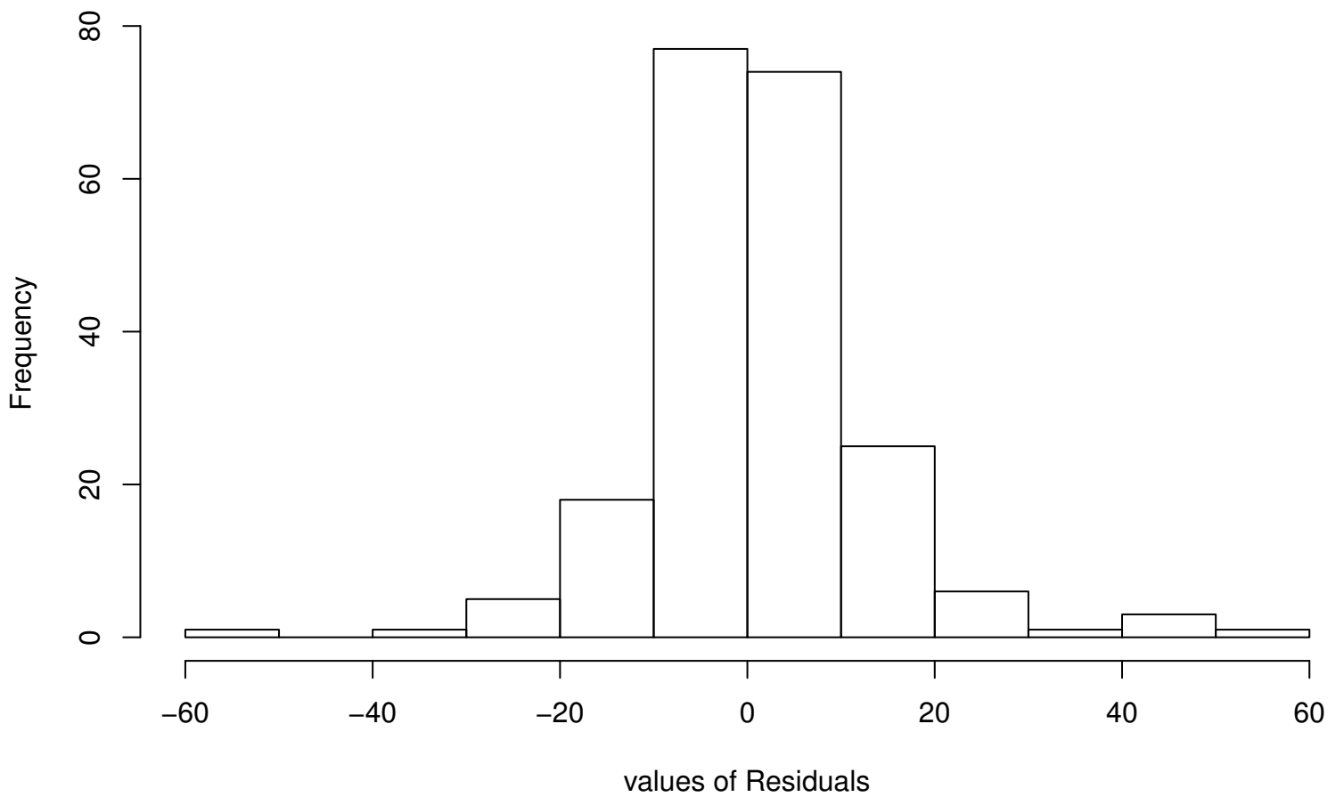
Residual Histogram
