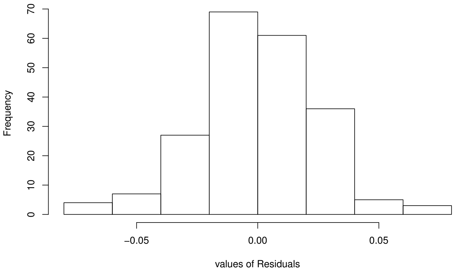
Residual Histogram
