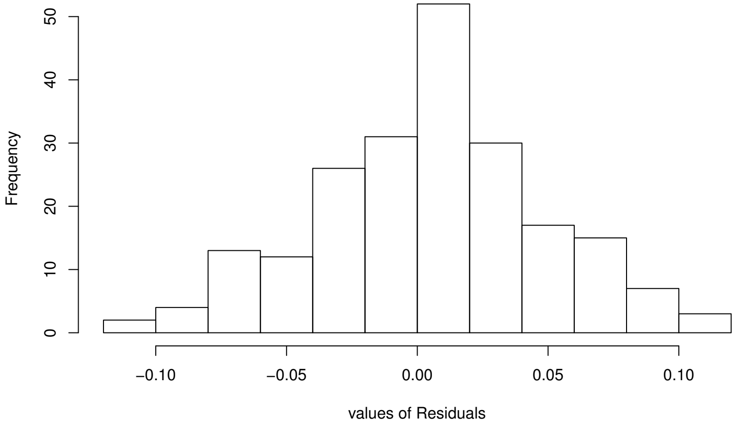
Residual Histogram
