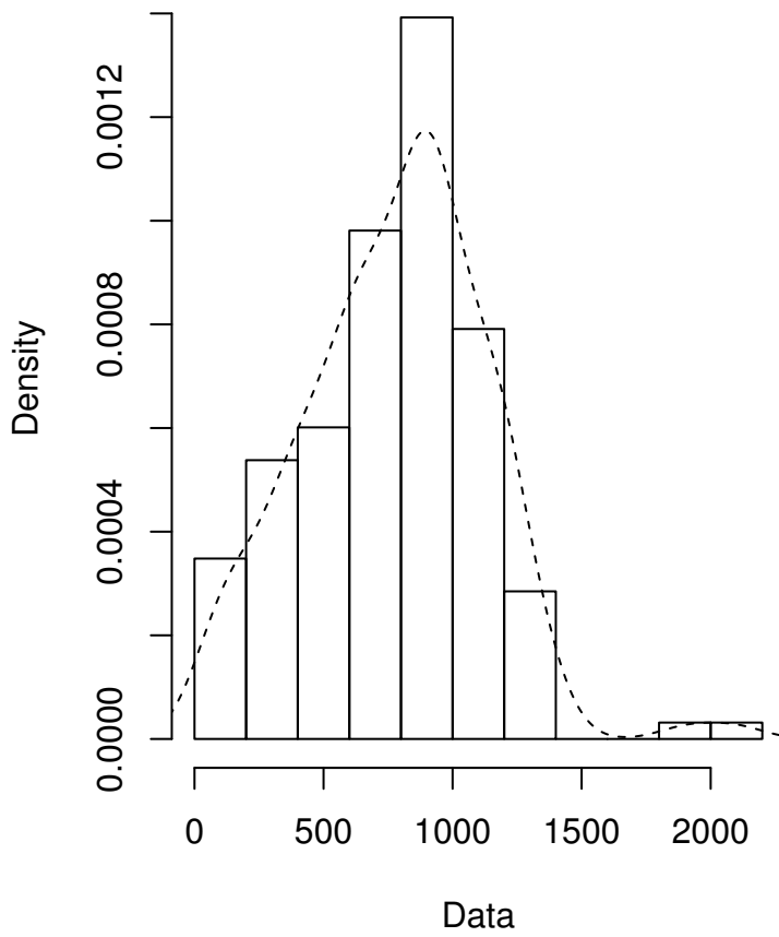
Empirical density
