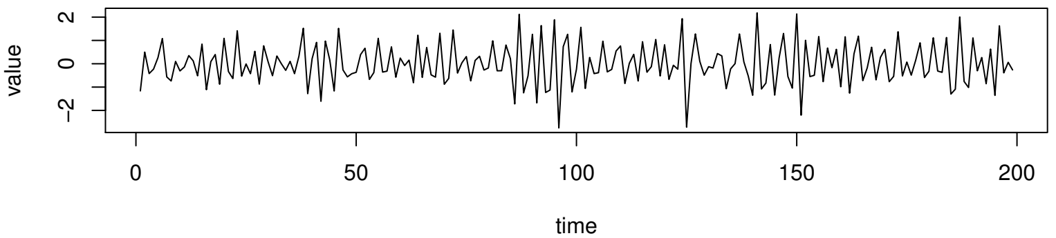
Working Time Series ( \lambda=0.6 , d=1 , D=1 )
