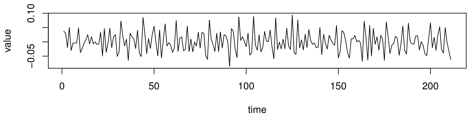
Working Time Series ( \lambda=-0.3 , d=1 , D=0 )
