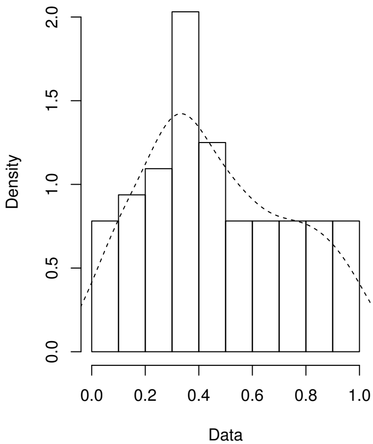
Empirical density
