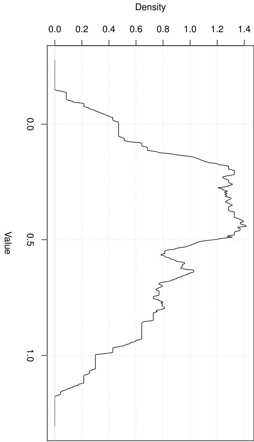
Rectangular Kernel
