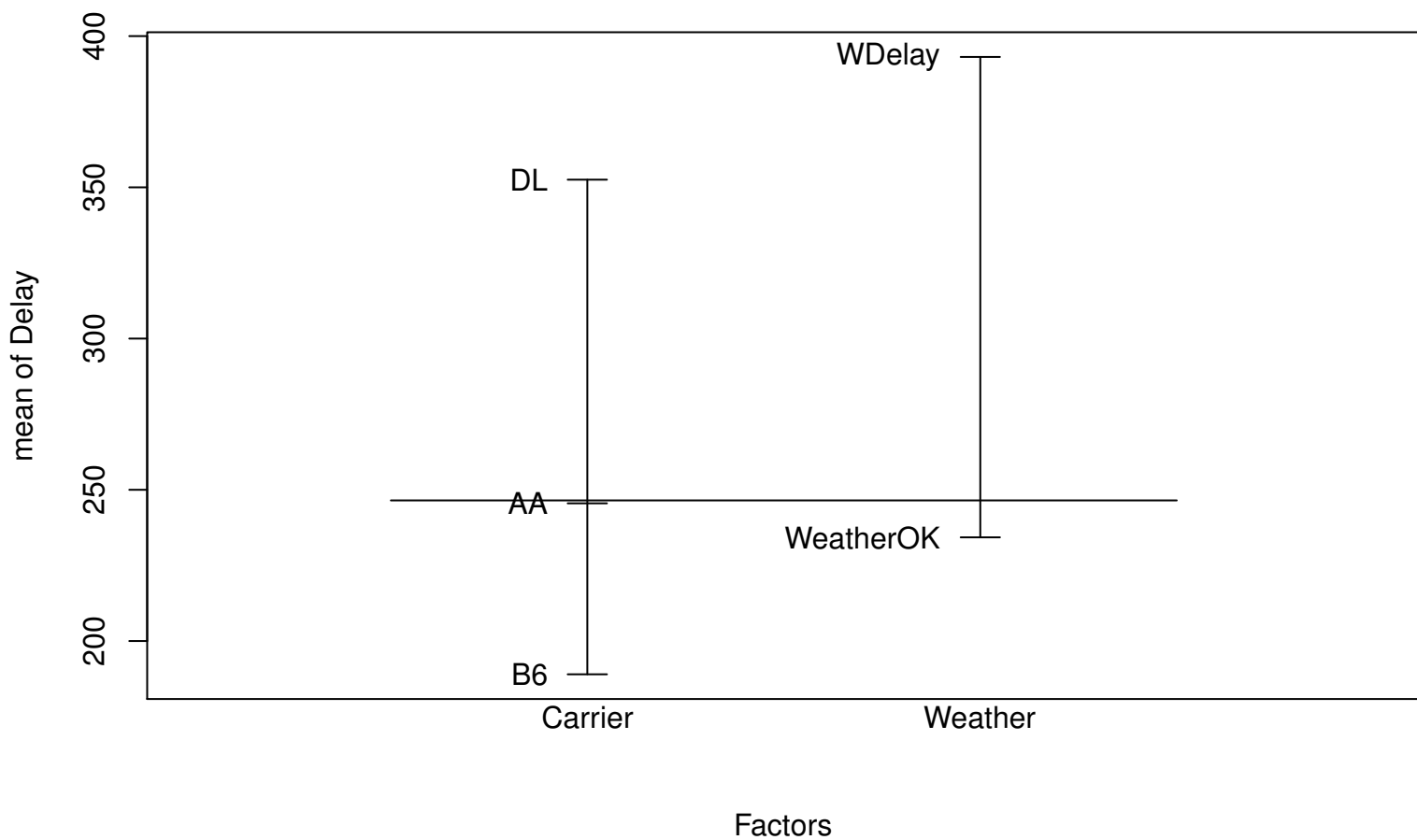
Design Plot of Group Means
