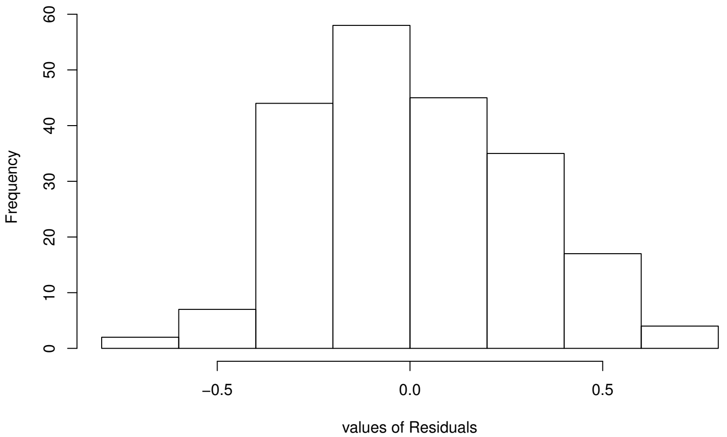
Residual Histogram
