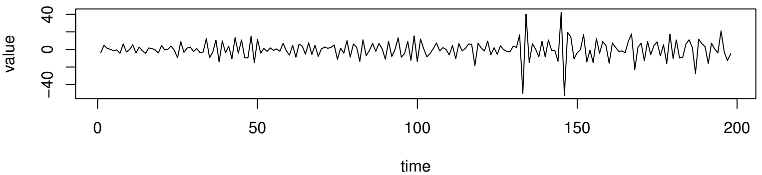
Working Time Series ( \lambda=1 , d=2 , D=1 )
