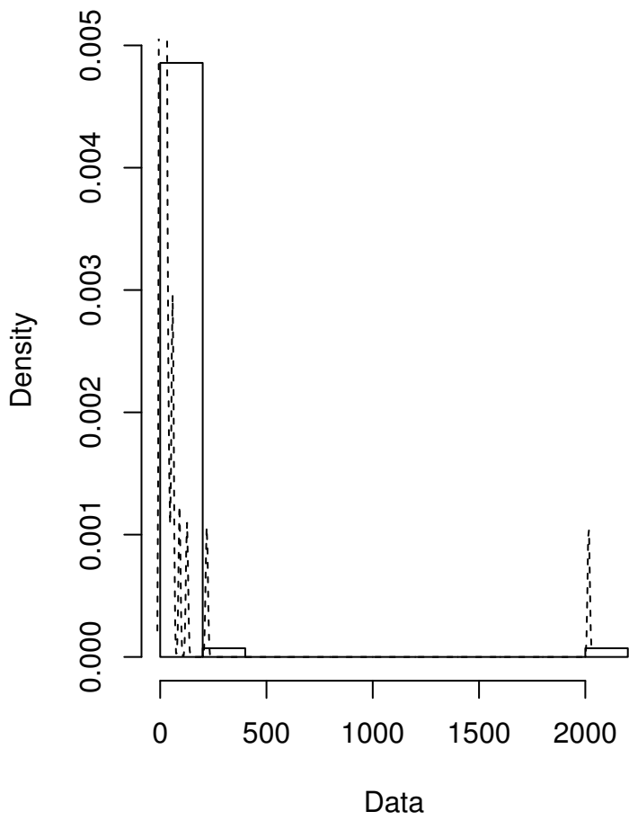
Empirical density
