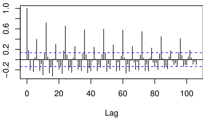
Residual ACF
