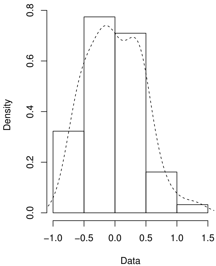
Empirical density
