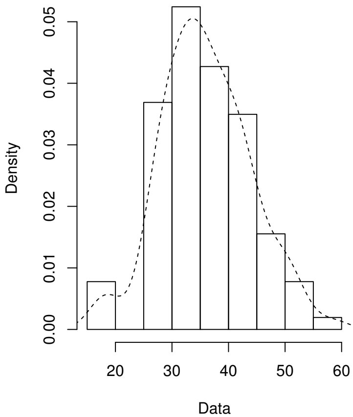
Empirical density
