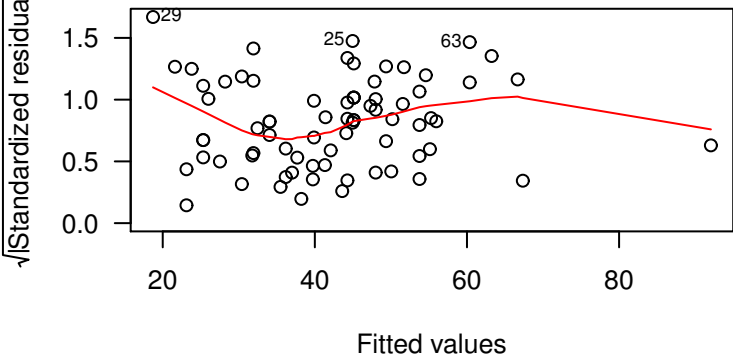
Scale-Location
