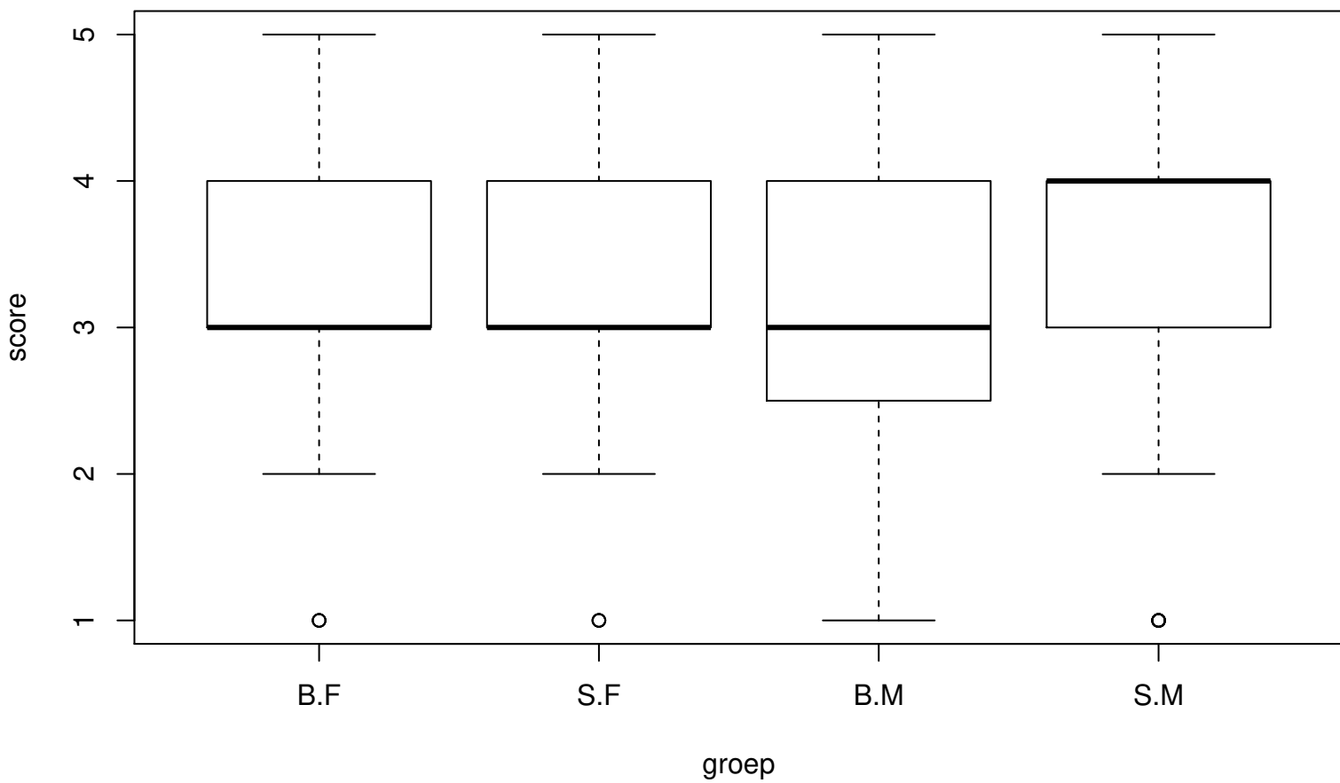
Boxplots of ANOVA Groups
