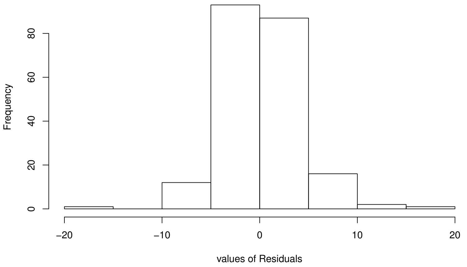
Residual Histogram
