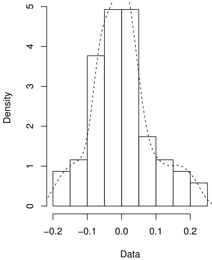
Empirical density
