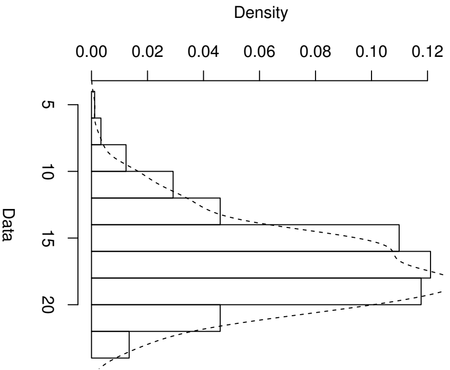
Empirical density
