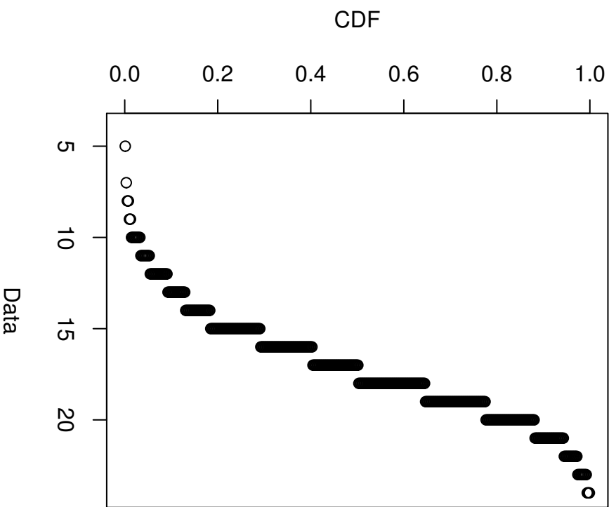
Cumulative distribution
