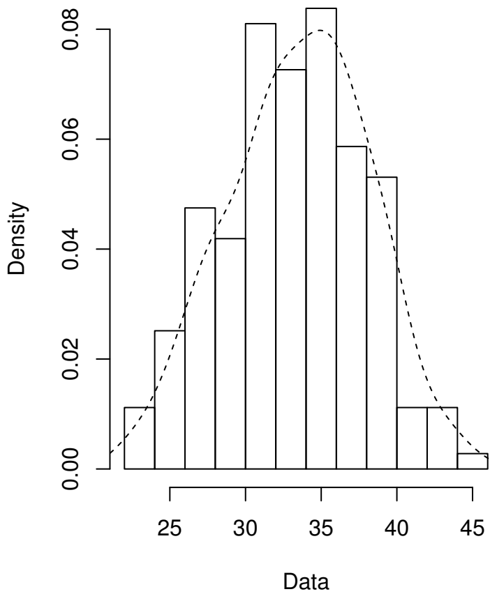
Empirical density
