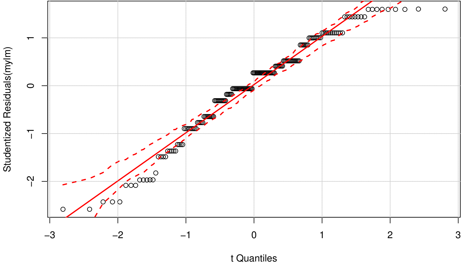
QQ Plot
