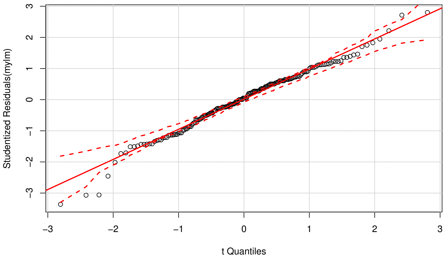
QQ Plot
