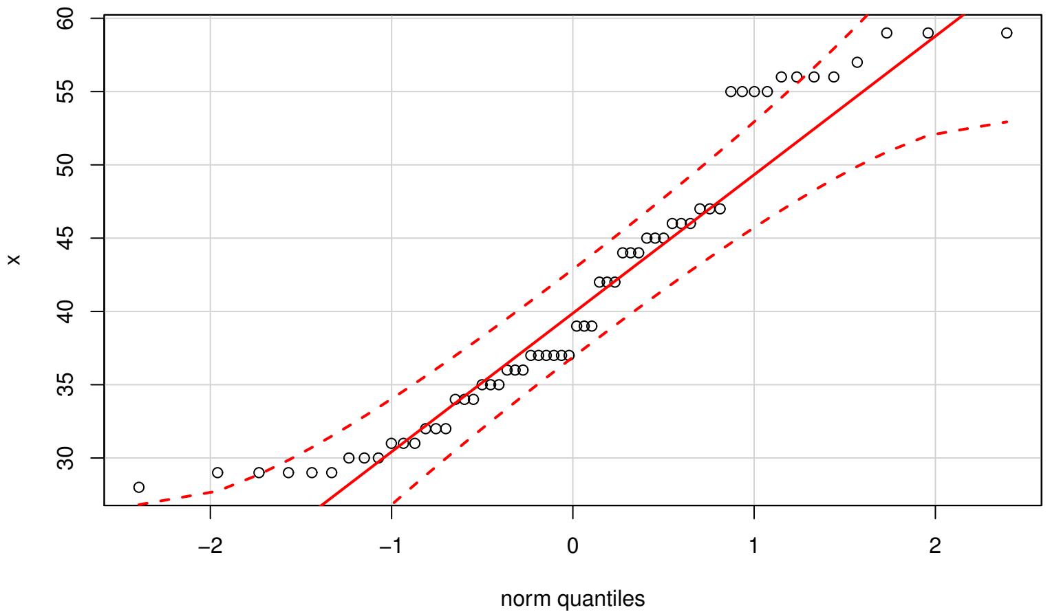
QQplot of variable x
