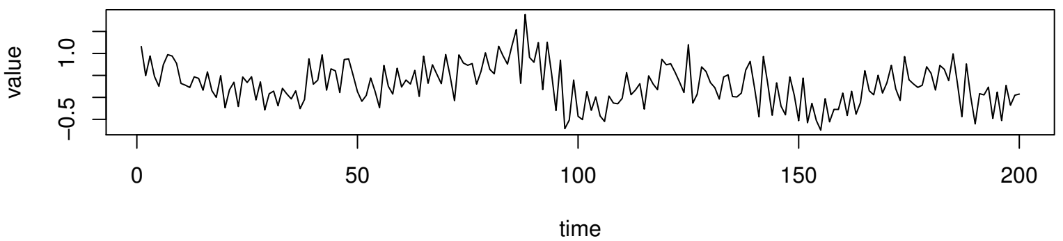
Working Time Series ( \lambda=0.5 , d=0 , D=1 )
