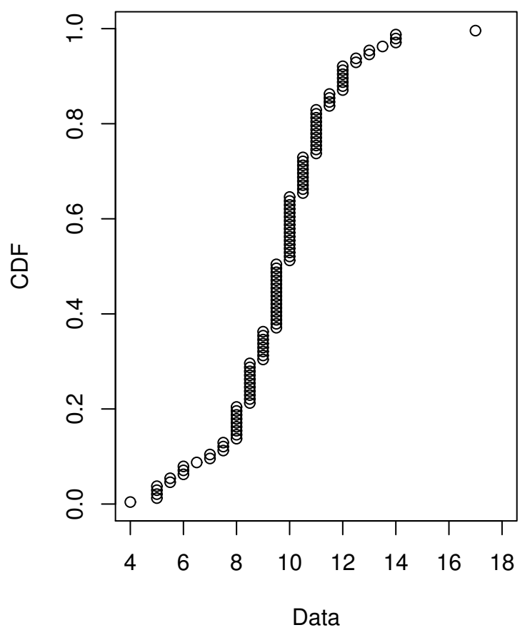
Cumulative distribution
