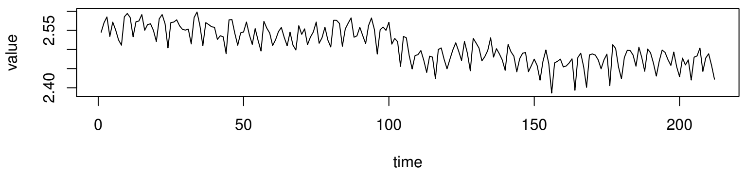
Working Time Series ( \lambda=-0.3 , d=0 , D=0 )
