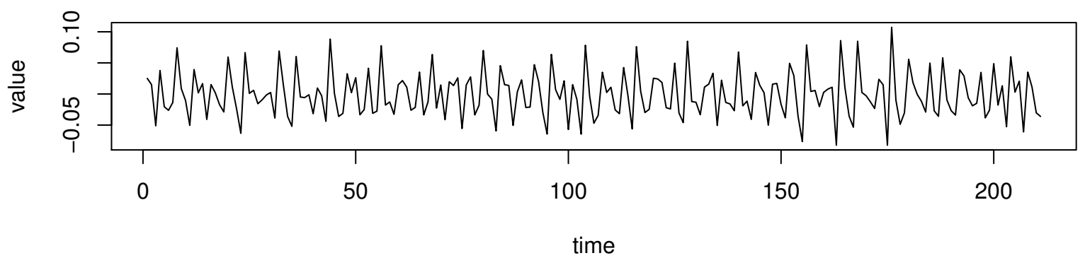
Working Time Series ( \lambda=-0.3 , d=1 , D=0 )
