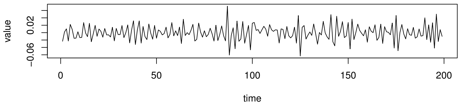
Working Time Series ( \lambda=-0.3 , d=1 , D=1 )
