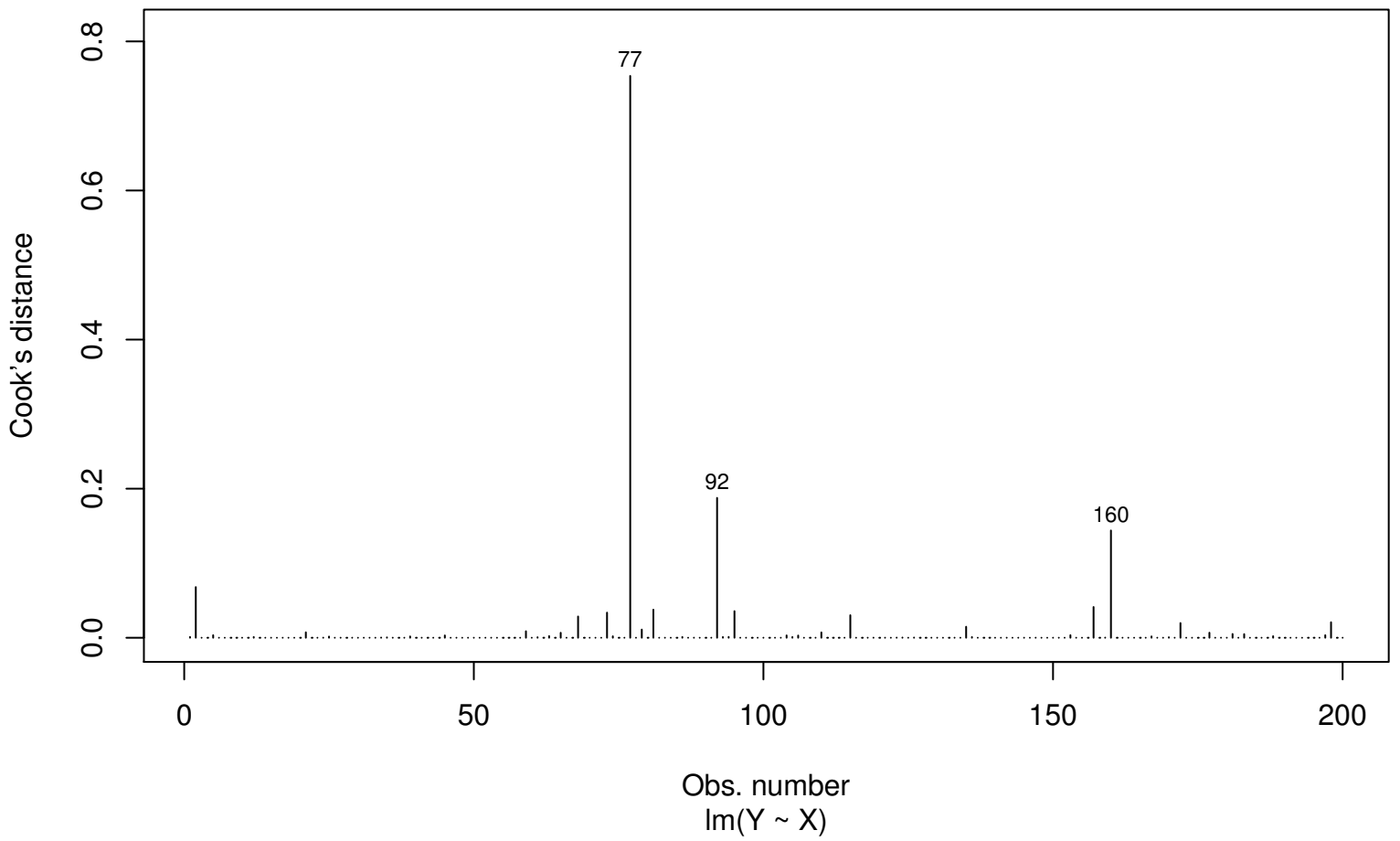
Cook's distance
