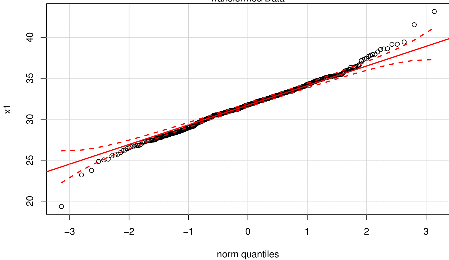
Transformed Data
