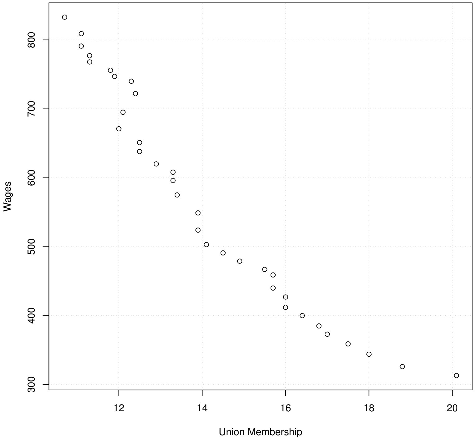
Scatterplot
