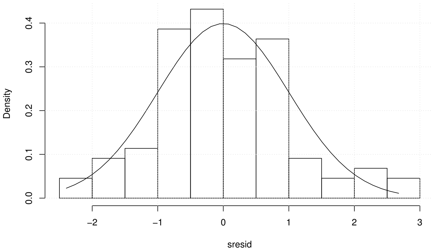
Distribution of Studentized Residuals
