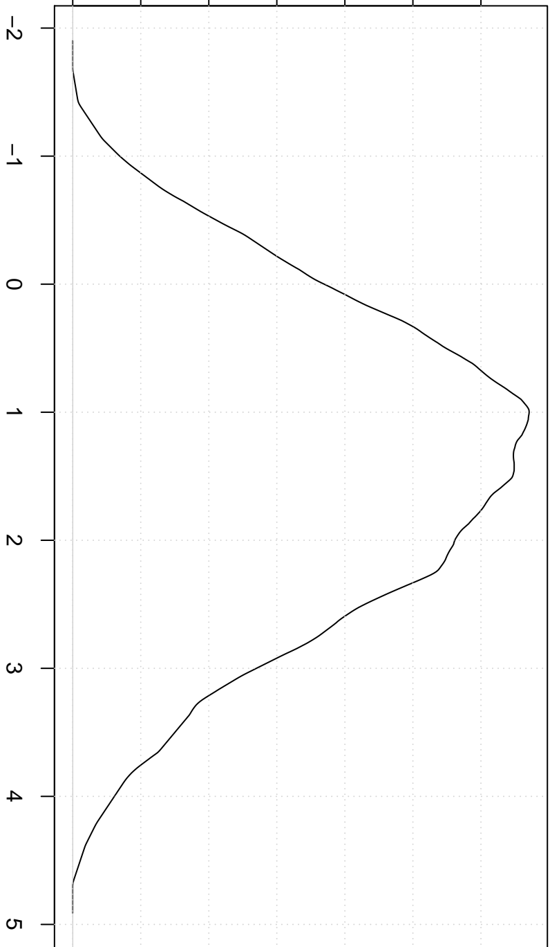
Triangular Kernel
