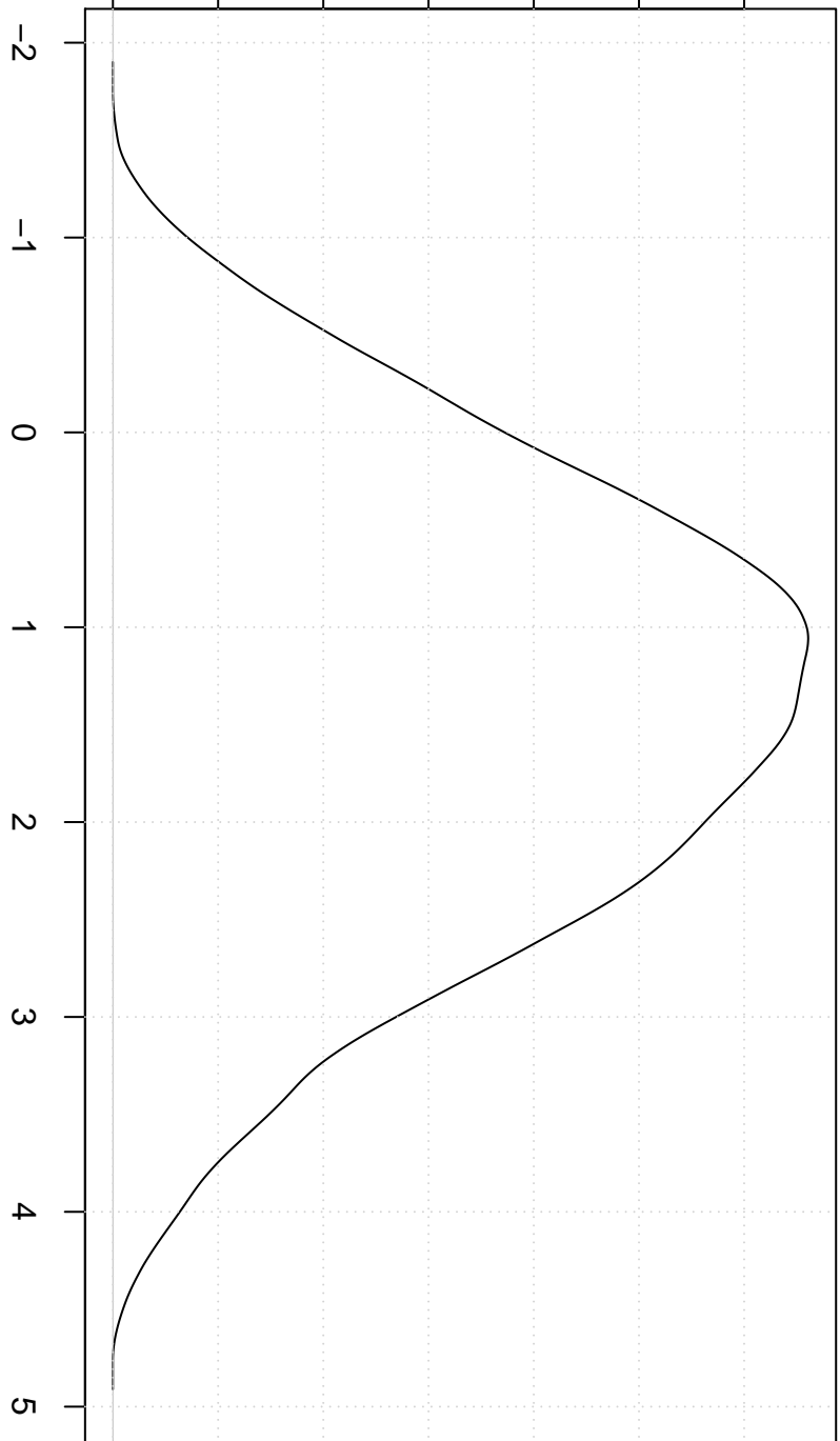
Biweight Kernel
