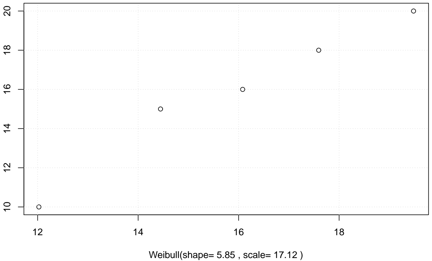
QQ plot (Weibull)
