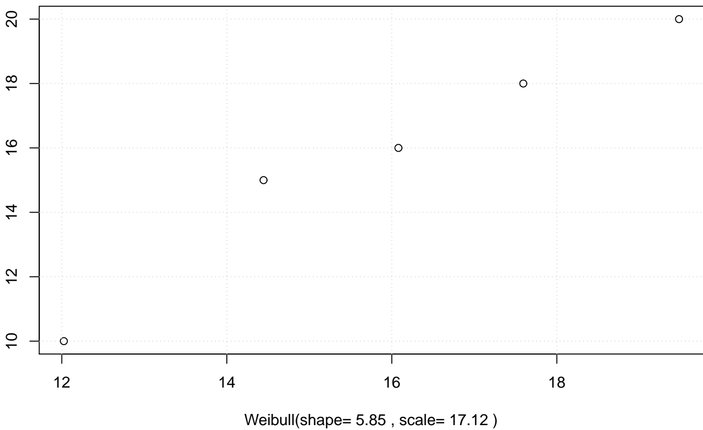
QQ plot (Weibull)
