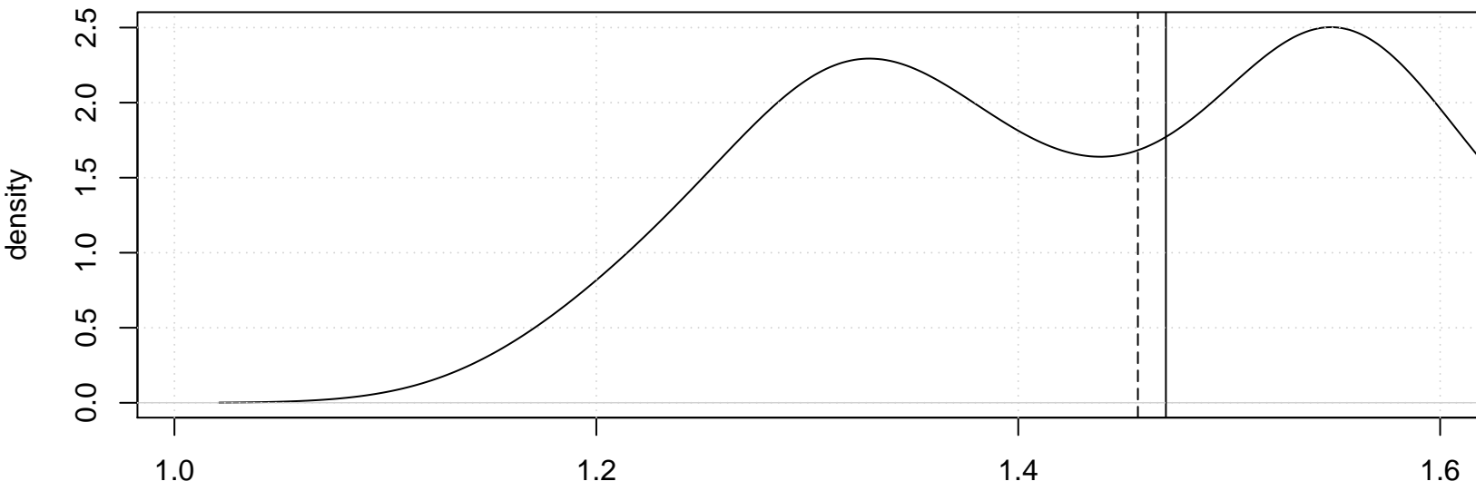
Density Plot – Gaussian Kernel
