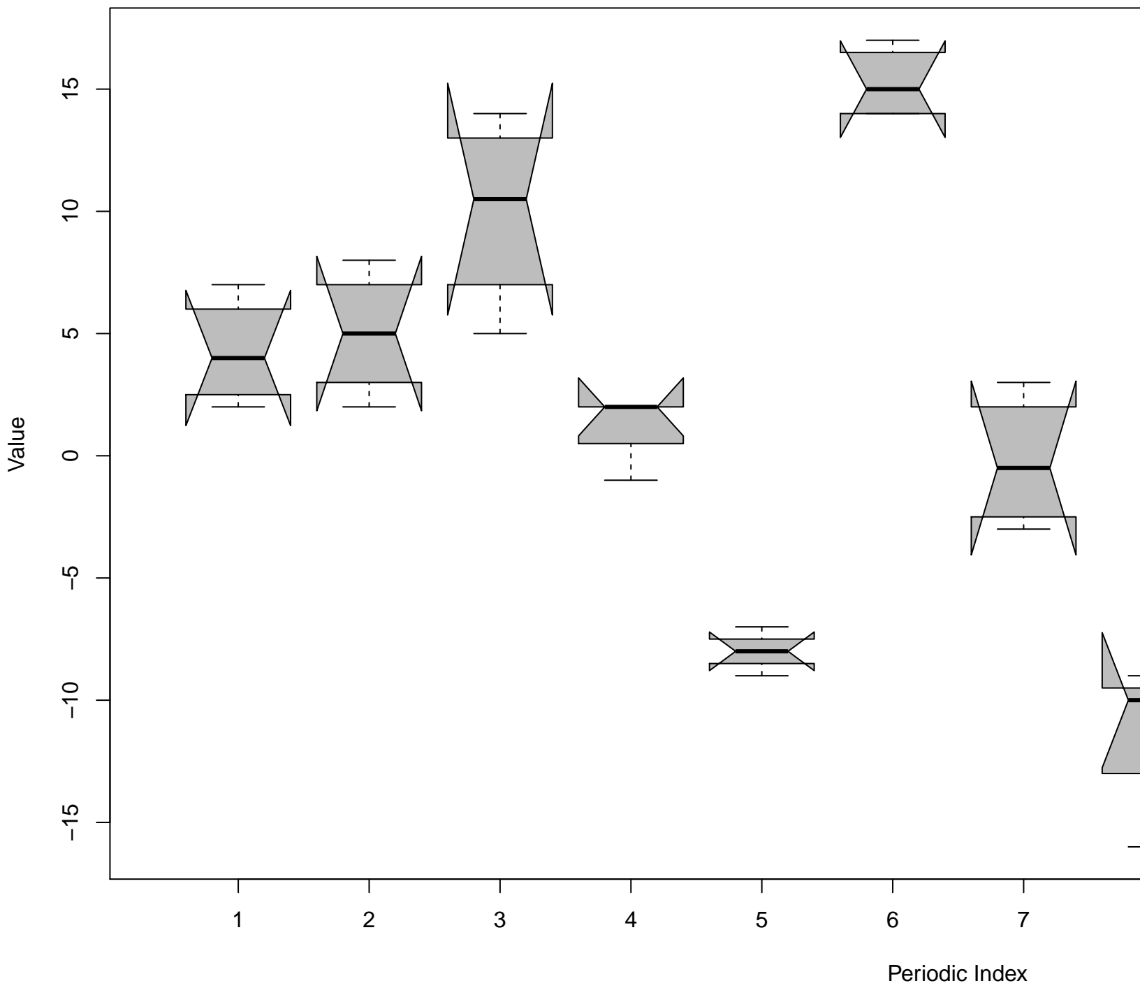
Notched Box Plots – Differenced Periodic
