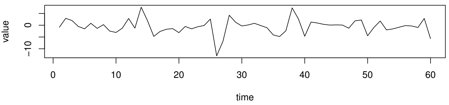
Working Time Series ( \lambda=0.4 , d=0 , D=1 )
