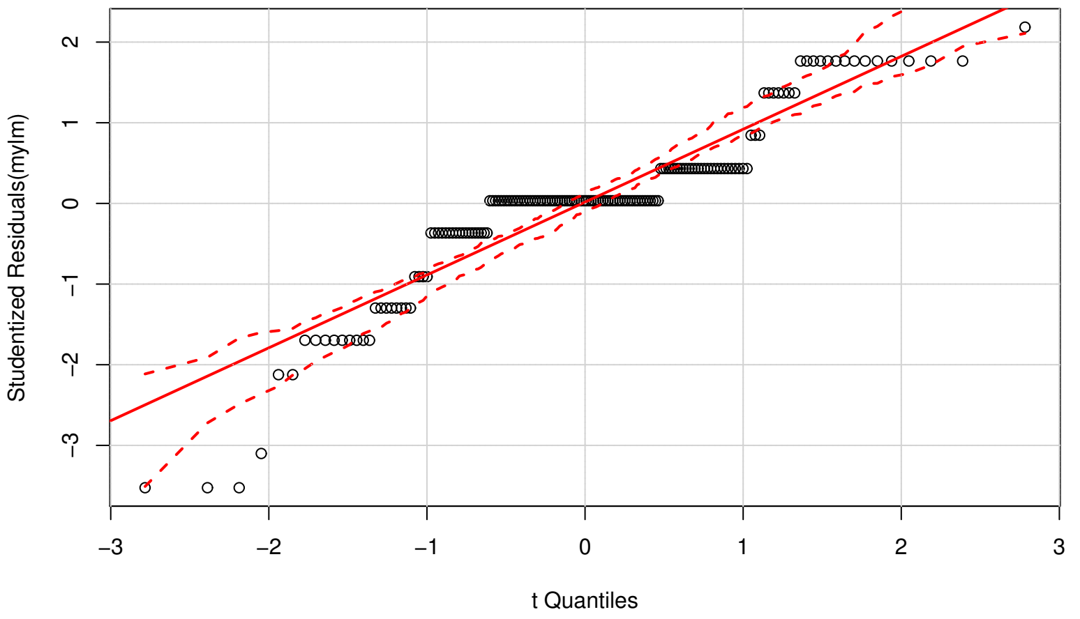
QQ Plot
