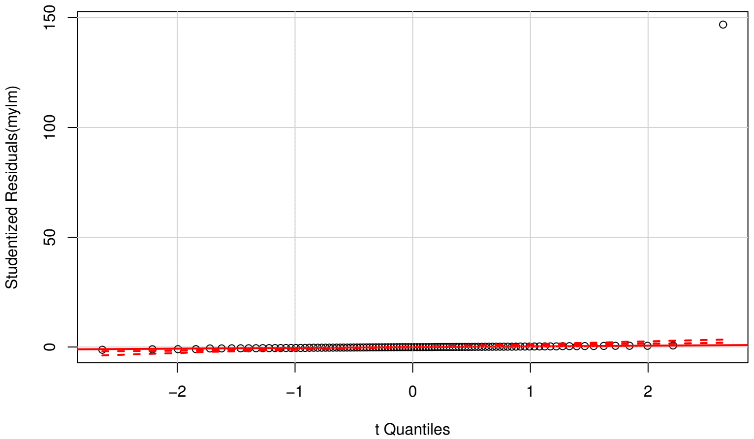
QQ Plot
