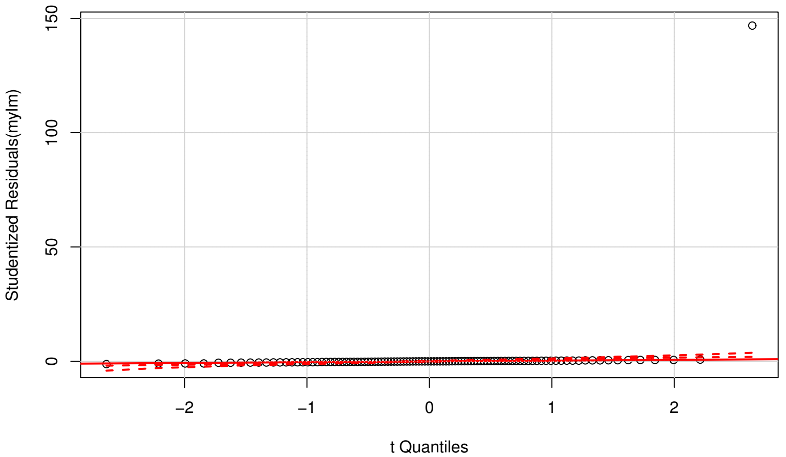
QQ Plot
