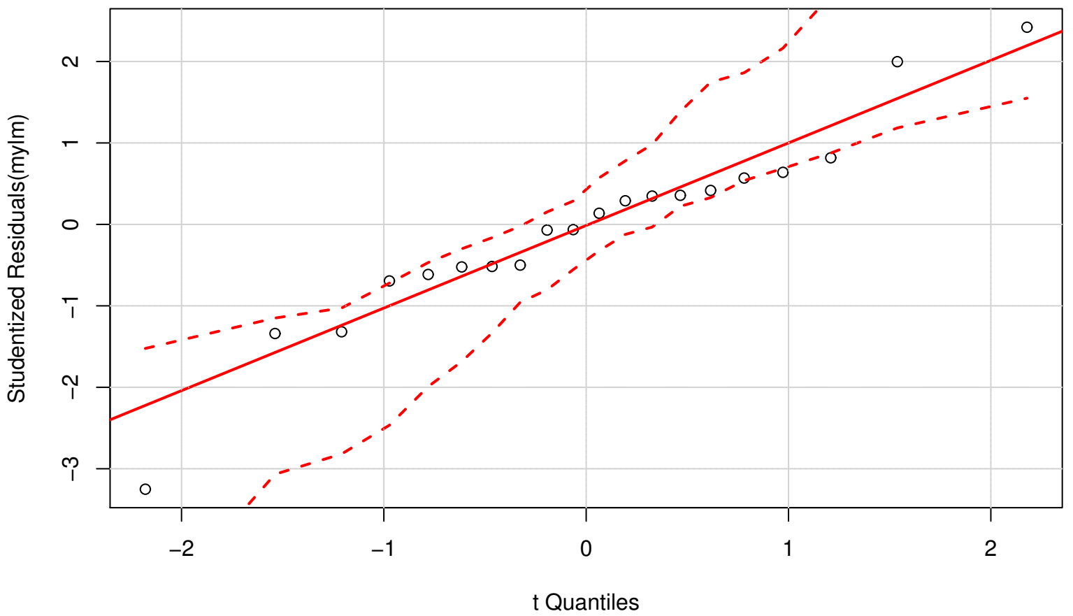
QQ Plot
