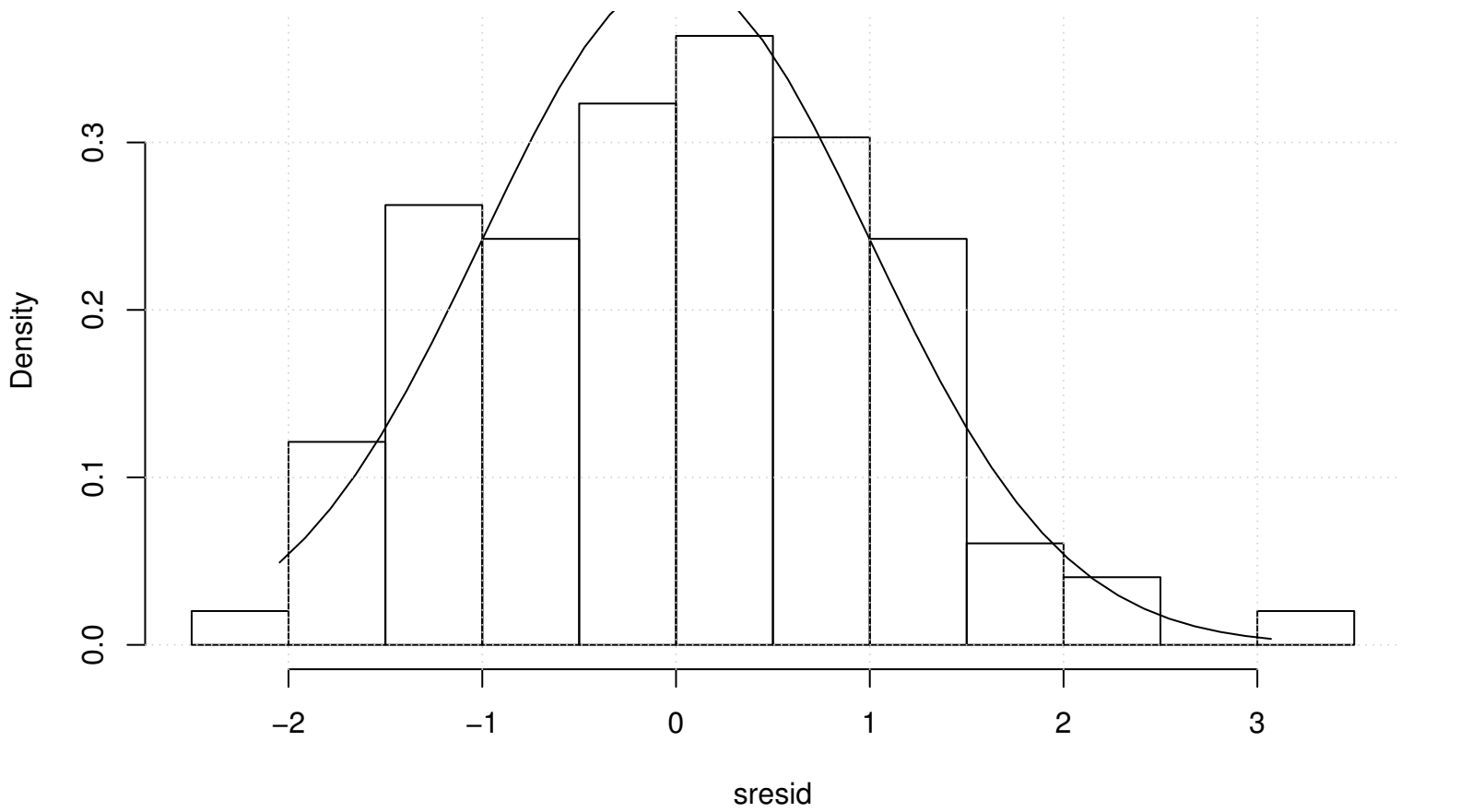
Distribution of Studentized Residuals
