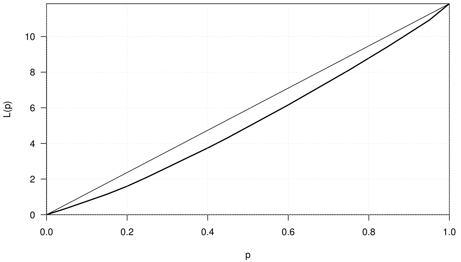
Lorenz curve
